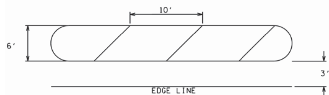
TYPICAL SECTION
